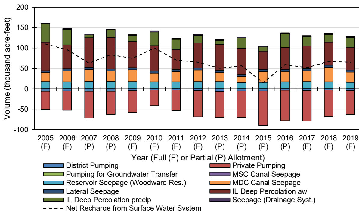
Figure 5-6. Groundwater System Inflows, Outflows, and Net Recharge (2005-2019)
