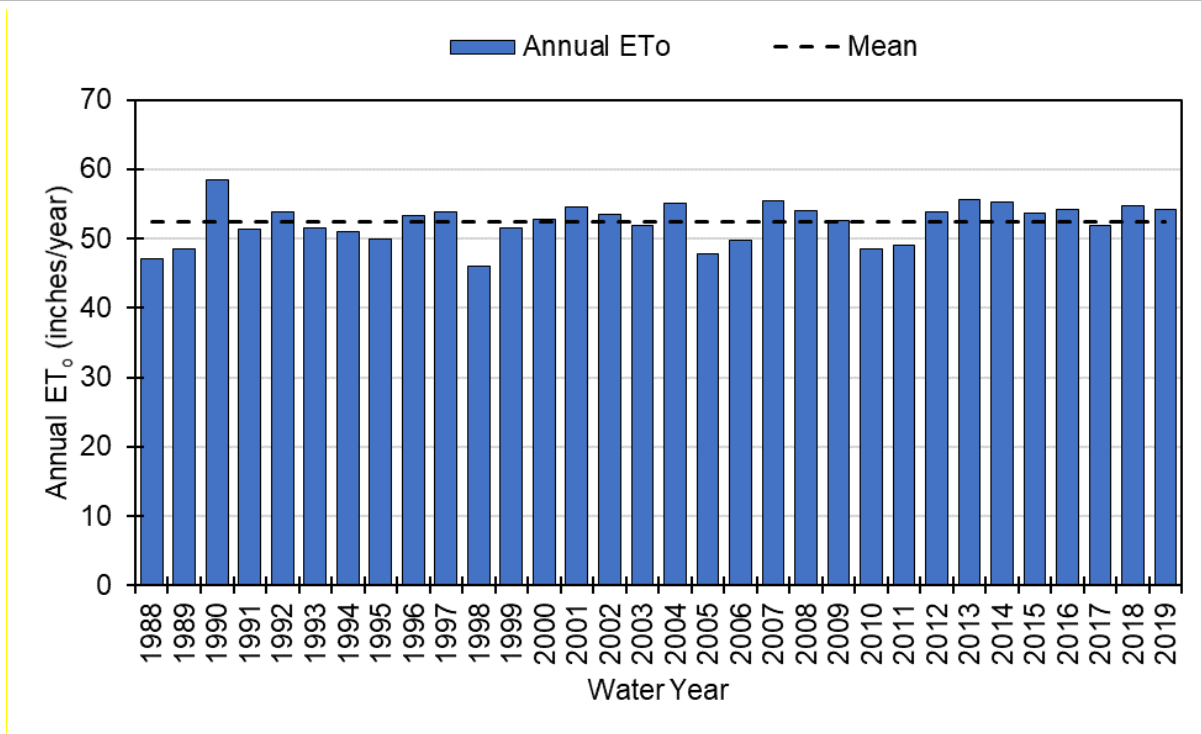
Figure 6-8. Historical Annual Reference ET at the Manteca CIMIS Station. 12
