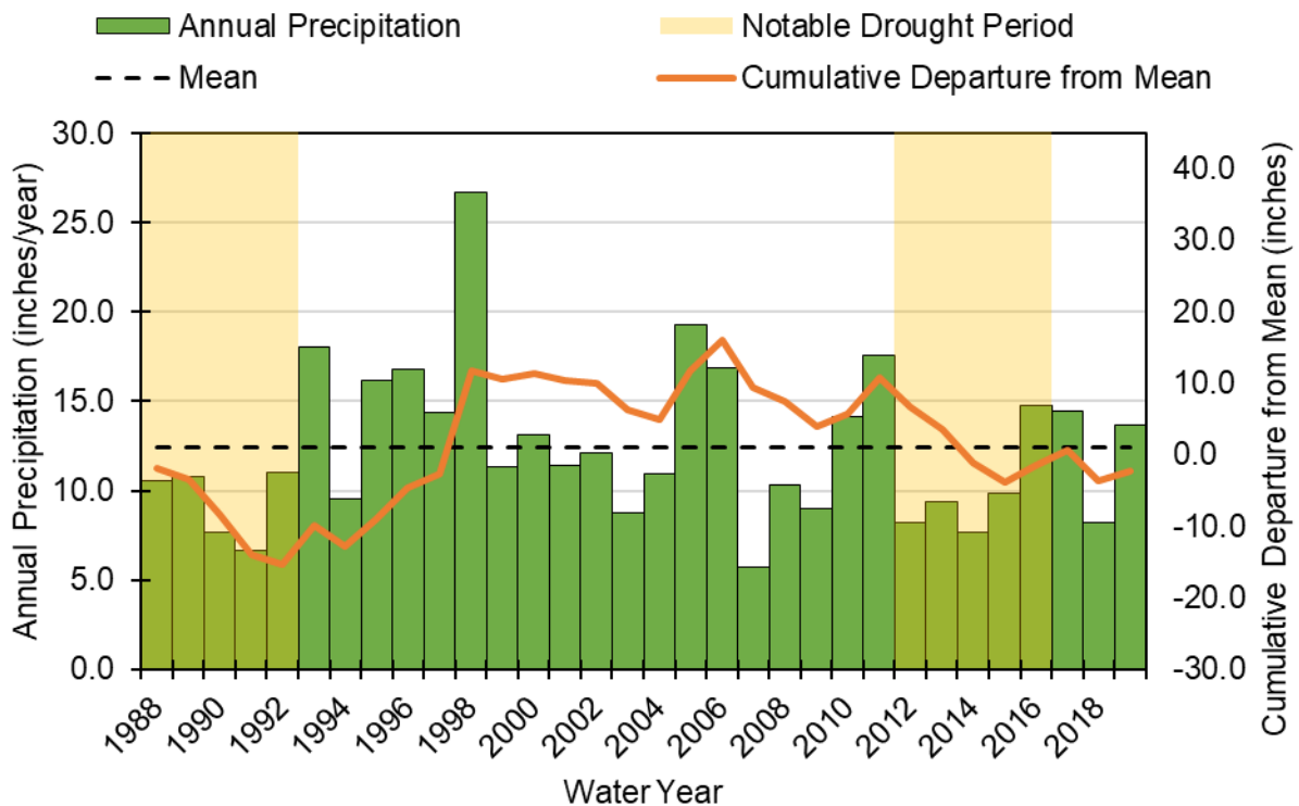
Figure 6-5. Historical Annual Precipitation and Cumulative Departure from the Mean Annual Precipitation at Manteca CIMIS Station.
