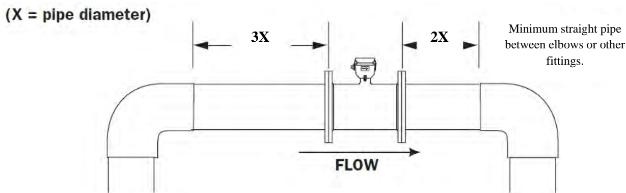
Figure C-1. Example Magnetic Flow Meter Installation.
